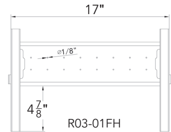
R03-01FH Front View
