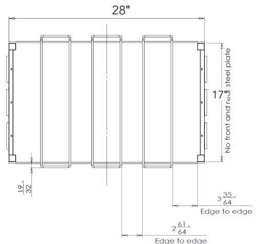
R03-02FV Top View
